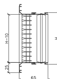
PB 2565-1H+R
