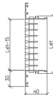
PB 3040-1H+R
