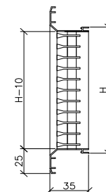
PB 2565-1H+R
