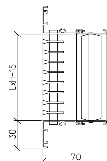
PB 3040-1H+R
